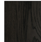
Morel (66M)
