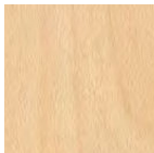
Natural (11M)
