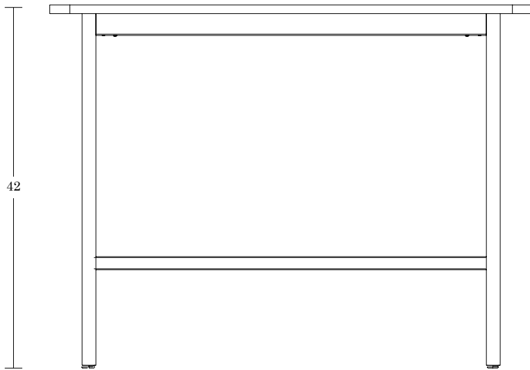
Fixed Bar Table 30x60 / FXT-3060-42
