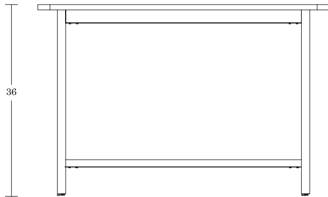
Fixed Counter 30x60 / FXT-3060-36
