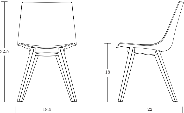
Wood Base / AMW
