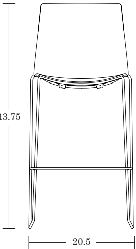
Sled Base Bar Chair / AMBS
