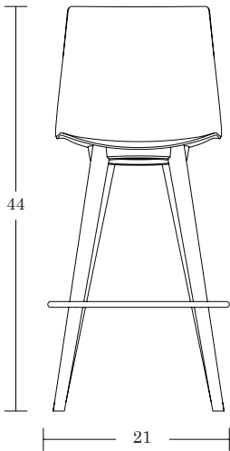
Wood Base Bar Chair/ AMBW
