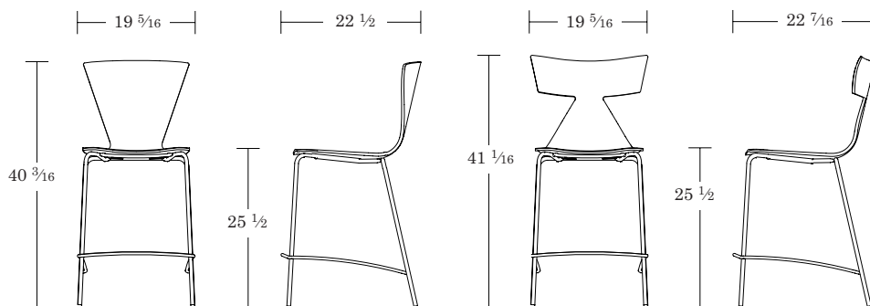
Galette Counter Chair / GLC + Upholstered Seat Onlay / GLCU
