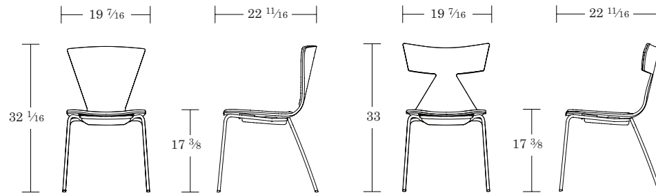
Galette Side Chair / GLS + Upholstered Seat Onlay / GLSU
