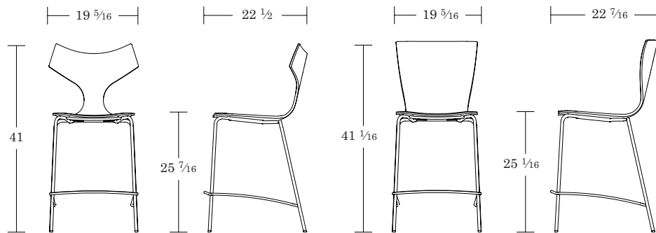
Tarte Counter Chair / TTC + Upholstered Seat Onlay / TTCU
