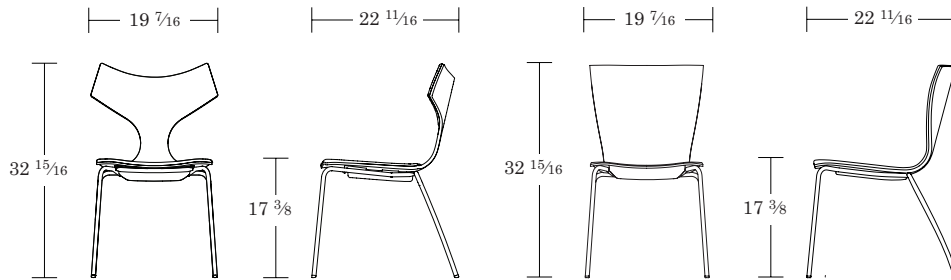
Tarte Side Chair / TTS + Upholstered Seat Onlay / TTSU
