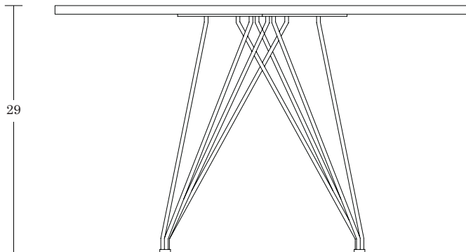
Large Radiant Base / MLRB
