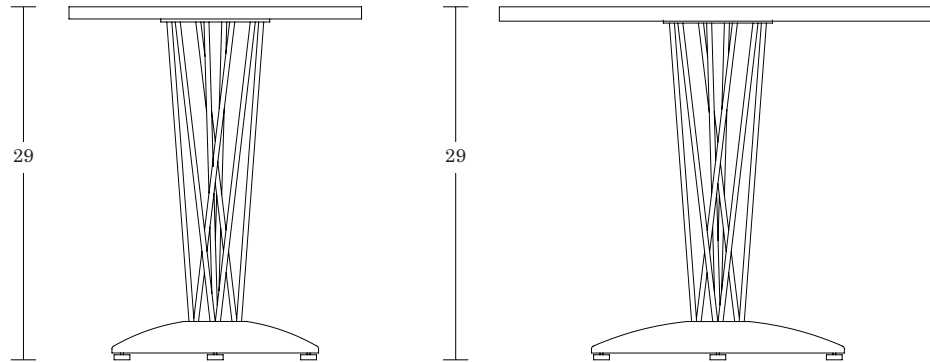
Small Dome Base / MSDB
